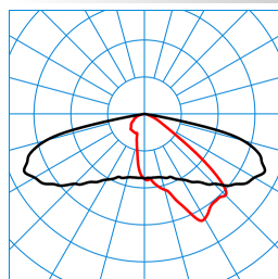
LIQ 50N-AB2L-LR/510/560/620-740 6G1 ET (CLO end value) TX278120
