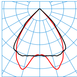
SFlow C1-L MRX LED3200-840 01 TX051985
