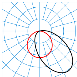
Sanesca W2 LED2600-840 03 (reading light) TX371845
