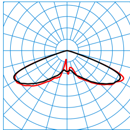
Publisca P2-RB6L-LR/2400-730 3G1S ET (CLO initial value) TX301745 ■ C0 - C180 ■ C90 - C270 DIN 5040: A20 UTE: 1,00 J CEN Flux Code: 20 57 98 100 100
