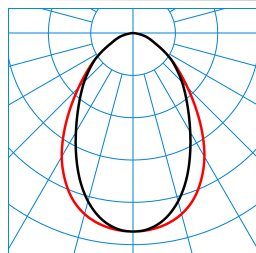
ArimoFit M48 DW19 IP 53-840 ETDD TX149915
