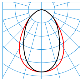
ArimoFit M48 DW19 IP 53-840 ETDD + ArimoFit Sky M48-TS ZER TX426319
