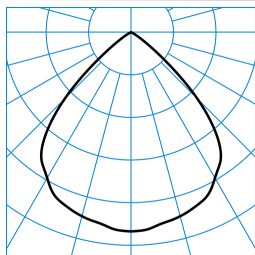
InperiaL G2 C07 BR22 2700-830 03 ■ C0 - C180 TX052911
