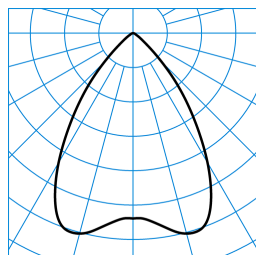
InperlaL G2 C07 BR22 3800-830 01 + RG-PC ■ C0 - C180 TX373497
