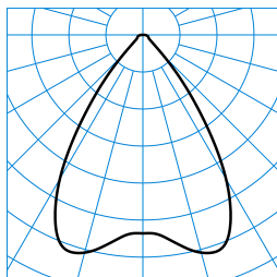
InperiaL G2 C07 BR22 3800-830 01 + ZN-PC ■ C0 - C180 TX373496
