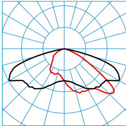
LIQ 70N-AB7L-LRA/10000-727 12G1 ETDD(CLO initial value) TX27826
