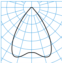
InperiaL G2 C07 BR19 1800-840 01 + ZN-PC ■ C0 - C180 TX372407
