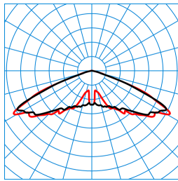
Publisca P1W-RB6L-LR/1800-730 2G1S TX053527
