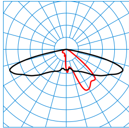
Publisca P1W-AB2L-LRA/2600-730 3G1S ET (CLO end value) TX301647
