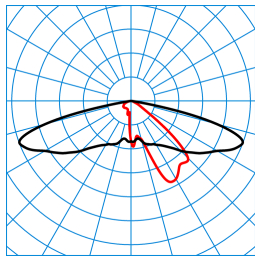
Publisca P1W-AB2L-LRA/2600-730 3G1S TX053499
