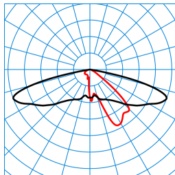
Publisca P1W-AB2L-LRA/2600-730 3G1S ET (CLO initial value) TX300916
