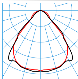
SFlow D1-L MRW LED3200-830 03 TX050958
