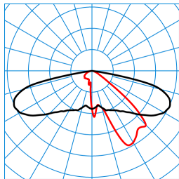
Publisca P2-AB2L-LRA/2400-740 3G1S TX047787 DIN 5040: A30 UTE: 1,00 l CEN Flux Code: 34 71 96 100 100
