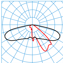
Publisca P2-AB2L-LRA/2400-740 3G1S ET (CLO end value) TX300800 DIN 5040: A30 UTE: 1,00 l CEN Flux Code: 34 71 96 100 100
