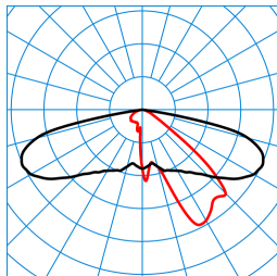
Publisca P2-AB2L-LRA/2400-740 3G1S ET (CLO initial value) TX301517 DIN 5040: A30 UTE: 1,00 l CEN Flux Code: 34 71 96 100 100
