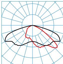
LIQ 70N-AB7L-LR/75/82/91-722 10G1 ET (CLO end value) TX281008
