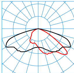
LIQ 70N-AB7L-LR/75/82/91-722 10G1 ET (CLO initial value) TX280968
