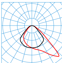
Bicult Act T COM TGCS 5500 I KL 03 EU (ActDCW) TX095978 DIN 5040: A50 UTE: 1,00 D CEN Flux Code: 59 89 98 100 100 0 0 0 0 ■ C0 - C180 ■ C90 - C270
