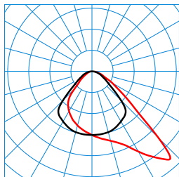
Bicult Act T COM TGCS 5500 I KL 03 EU (ActDWW) TX095980 DIN 5040: A54 UTE: 1,00 D CEN Flux Code: 59 89 98 100 100 0 0 0 0 ■ C0 - C180 ■ C90 - C270
