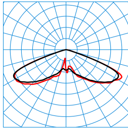
Publisca P1-RB6L-LRA/2200-740 3G1S ET (CLO initial value) TX301939 ■ C0 - C180 ■ C90 - C270 DIN 5040: A20 UTE: 1,00 J CEN Flux Code: 20 57 98 100 100
