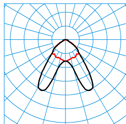
E-Line Fi LightP DA-B-DA 65-830 L75 03 (225) TX372113
