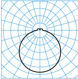
Olisq RWD2 DW 20-830 ETBLE +DMM IP54 PC TX375705
