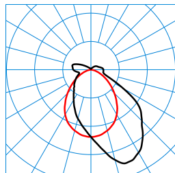
TugraHE Act 18 PAW 64-840 ETDD8 01 (ACTDCW) TX303336 ■ C0 - C180 ■ C90 - C270 DIN 5040: B40 UTE: 0,87 E + 0,13 T CEN Flux Code: 48 79 93 87 100 7 25 60 13
