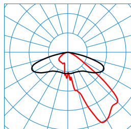
Publisca P2-AB2L-LRA/2900-740 4G1S ET (CLO initial value) TX300909 ■ C0 - C180 ■ C90 - C270 DIN 5040: A30 UTE: 1,00 G CEN Flux Code: 35 73 97 100 100
