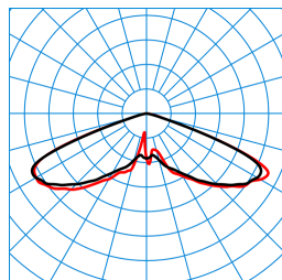
Publisca P2-RB6L-LRA/2200-740 3G1S ET (CLO initial value) TX301773 ■ C0 - C180 ■ C90 - C270 DIN 5040: A20 UTE: 1,00 J CEN Flux Code: 20 57 98 100 100
