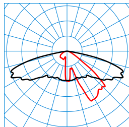
Publisca P1W-AB2L-LR/1500-730 2G1S ET (CLO end value) TX300604 DIN 5040: A30 UTE: 1,00 l CEN Flux Code: 32 69 96 99 100 0 17 50 1
