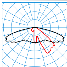
Publisca P1W-AB2L-LR/1500-730 2G1S TX053477 DIN 5040: A30 UTE: 1,00 l CEN Flux Code: 32 69 96 99 100 0 17 50 1
