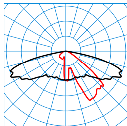
Publisca P1W-AB2L-LR/1500-730 2G1S ET (CLO initial value) TX300235 DIN 5040: A30 UTE: 1,00 l CEN Flux Code: 32 69 96 99 100 0 17 50 1
