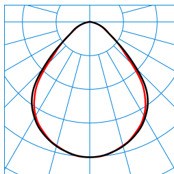
Opendo D2-L PW19 20-47/5/ML-840 ET 03 (3500lm) TX376540
