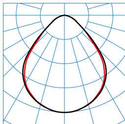
Opendo D2-L PW19 20-47/5/ML-840 ET 03 (2500lm) TX376538
