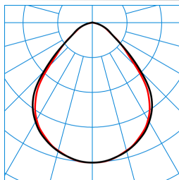
Opendo D2-L PW19 20-47/5/ML-840 ET 03 (2000lm) TX376537
