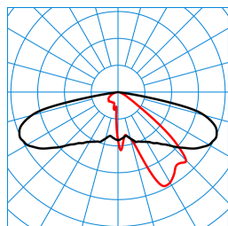
Publisca P2-AB2L/2000-730 3G1S ETDD (CLO end value) TX300404
