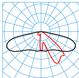
Publisca P2-AB2L-LRA/1650-730 2G1S ET (CLO initial value) TX300574 ■ C0 - C180 ■ C90 - C270 DIN 5040: A30 UTE: 1,00 G CEN Flux Code: 34 70 96 100 100
