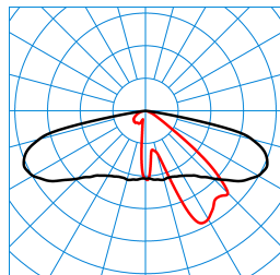
Publisca P2-AB2L-LRA/1650-730 2G1S ET (CLO end value) TX300574 ■ C0 - C180 ■ C90 - C270 DIN 5040: A30 UTE: 1,00 G CEN Flux Code: 34 70 96 100 100
