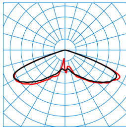
Publisca P2-RB6L-LR/2000-730 3G1S TX047856 DIN 5040: A20 UTE: 1,00 J CEN Flux Code: 20 57 98 100 100
