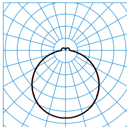
Olisq Act QWD2 DW 35 ETDD8 (ActDSU) TX375673
