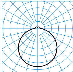
Olisq Act QWD2 DW 35 ETDD8 (ActDCW) TX376155
