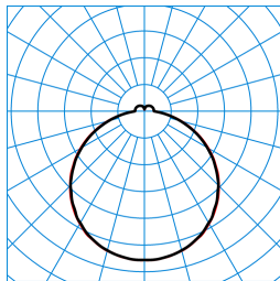
Olisq Act QWD2 DW 35 ETDD8 (ActDWW) TX376245
