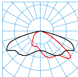
LIQ 70N-AB7L-SLR2/14500-727 12G1 ET (CLO initial value) TX278031
