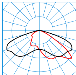
9711SG-AB7L/51/62/75-740 8G2 (7500 lm) TX064265 DIN 5040: A30 UTE: 1,00 H CEN Flux Code: 35 74 98 100 100
