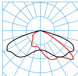
9711SG-AB7L/51/62/75-740 8G2 (6200 lm) TX064264 DIN 5040: A30 UTE: 1,00 H CEN Flux Code: 35 74 98 100 100
