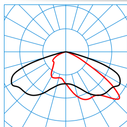
9711SG-AB7L/51/62/75-740 8G2 (5100 lm) TX064263 DIN 5040: A30 UTE: 1,00 H CEN Flux Code: 35 74 98 100 100
