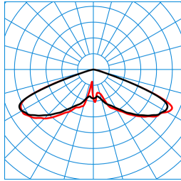
Publisca P1-RB6L-LRA/2400-730 3G1S TX047669 DIN 5040: A20 UTE: 1,00 J CEN Flux Code: 20 57 98 100 100
