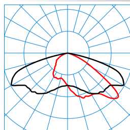
LIQ 70N-AB7L-LR/8200-730 10G1 ET (CLO end value) TX278171
