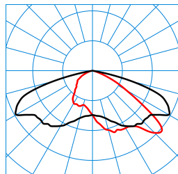
LIQ 70N-AB7L-LR/8200-730 10G1 ET (CLO initial value) TX278323
