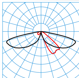
LTX Z-AB2L-LRA/15/18/26-740 4G1 (1800 lm) TX062709 DIN 5040: A20 UTE: 1,00 l CEN Flux Code: 24 61 92 100 100 0 0 0 0 ■ C0 - C180 ■ C90 - C270
