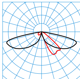
LTX Z-AB2L-LRA/15/18/26-740 4G1 (2600 lm) TX062710 DIN 5040: A20 UTE: 1,00 l CEN Flux Code: 24 61 92 100 100 0 0 0 0 ■ C0 - C180 ■ C90 - C270
