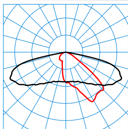
LIQ 50N-AB2L-LRA/22/26/32-730 4G1 ETDD (CLO end value) TX277677
