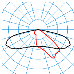
LIQ 50N-AB2L-LRA/22/26/32-730 4G1 ETDD (CLO initial value) TX277995
