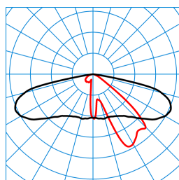
Publisca P2-AB2L-LRA/1000-740 2G1S ET (CLO initial value) TX300328 ■ C0 - C180 ■ C90 - C270 DIN 5040: A30 UTE: 1,00 G CEN Flux Code: 34 70 96 100 100
