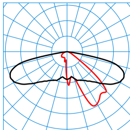
Publisca P1-AB2L-LR/2600-730 3G1S ET (CLO initial value) TX300848 ■ C0 - C180 ■ C90 - C270 DIN 5040: A30 UTE: 1,00 l CEN Flux Code: 34 71 96 100 100
