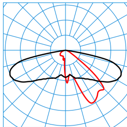
Publisca P1-AB2L-LR/2600-730 3G1S TX047523 ■ C0 - C180 ■ C90 - C270 DIN 5040: A30 UTE: 1,00 l CEN Flux Code: 34 71 96 100 100
