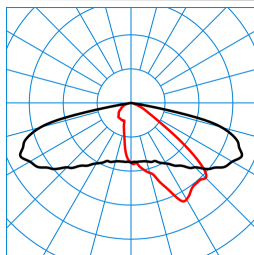
LIQ 50N-AB2L-LR/510/560/620-727 6G1 ET (CLO end value) TX278262
