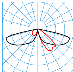
CS 19 100-AB2L-LR/3800-740 4G1S ET (CLO initial value) TX300029 DIN 5040: A20 UTE: 1,00 l CEN Flux Code: 27 65 96 100 100 0 0 0 0 ■ C0 - C180 ■ C90 - C270
