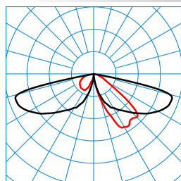
CS 19 100-AB2L-LR/3800-740 4G1S ET (CLO end value) TX300028 DIN 5040: A20 UTE: 1,00 l CEN Flux Code: 27 65 96 100 100 0 0 0 0 ■ C0 - C180 ■ C90 - C270
