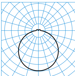
Olisq Act RWD4 DW 40 ETDD8 IP54 PC + Olisq RWD4 ZDR 1/2 03 (ActDWW) TX427400
