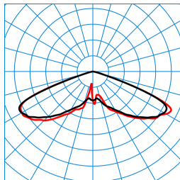
Publisca P1-RB6L-LR/2200-740 3G1S ET (CLO initial value) TX301729 ■ C0 - C180 ■ C90 - C270 DIN 5040: A20 UTE: 1,00 J CEN Flux Code: 20 57 98 100 100
