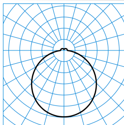
Olisq RWD3 DW 50-830 ETBLE +DMM PC TX375986
