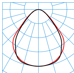
PareliaAct H-L 13000 +LM1 03 N8 (ActDCW) (LEO_direct_c90geo) TX370044
