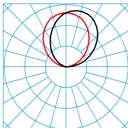
Sanesca W3-S2/R LED5000-840 03 (night light) TX372732
