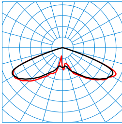
Publisca P1-RB6L-LRA/2000-740 3G1S ET (CLO initial value) TX300659 ■ C0 - C180 ■ C90 - C270 DIN 5040: A20 UTE: 1,00 J CEN Flux Code: 20 57 98 100 100
