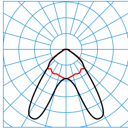
7651 LightP DA-B-DA 65-840ETDD L75 01 (225) TX557845
