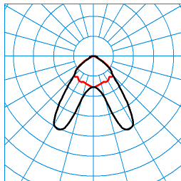
E-Line Fi LightP DA-B-DA 65-840 L75 01 (225) TX123794
