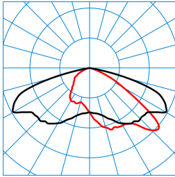
LIQ 70N-AB7L-LR/12000-722 12G1 ET (CLO end value) TX280973
