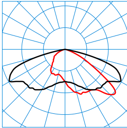
LIQ 70N-AB7L-LR/12000-722 12G1 ET (CLO initial value) TX280966
