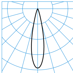
E-Line 7651 LentyP L-SP 30-BF M54 ETDD 05 (225) TX463524
