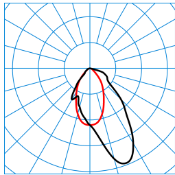
CreavoAct M46-TS LWW-03 42-8 ETDD8 01 (ACTDCW) TX195447 DIN 5040: A50 UTE: 1,00 C CEN Flux Code: 70 92 99 100 100 ■ C0 - C180 ■ C90 - C270
