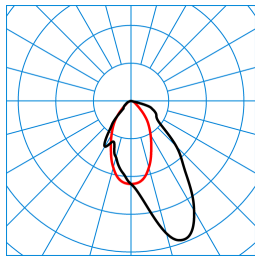
CreavoAct M46-TS LWW-03 42-8 ETDD8 01 (ACTDWW) TX195449 DIN 5040: A50 UTE: 1,00 C CEN Flux Code: 70 92 99 100 100 ■ C0 - C180 ■ C90 - C270
