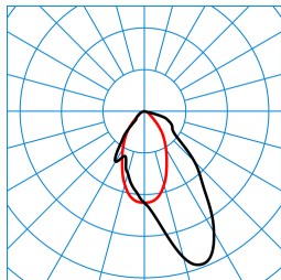
CreavoAct M46-TS LWW-03 42-8 ETDD8 01 (ACTDSU) TX195448 DIN 5040: A50 UTE: 1,00 C CEN Flux Code: 70 92 99 100 100 ■ C0 - C180 ■ C90 - C270
