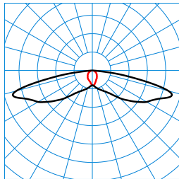
LIQ 50N-SB3L-SLR1/2200-722 2G1 ET (CLO initial value) TX280960
