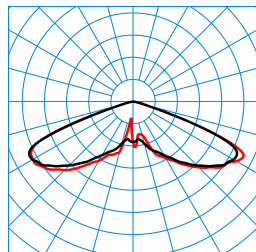
Publisca P2-RB6L-LR/2200-740 3G1S ET (CLO end value) TX301932 DIN 5040: A20 UTE: 1,00 J CEN Flux Code: 20 57 98 100 100
