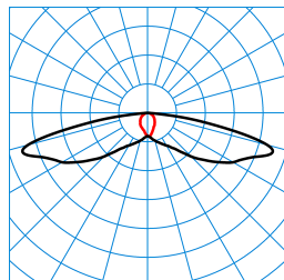
LIQ 50N-SB3L-LR/1000-722 2G1 ET (CLO initial value) TX281072
